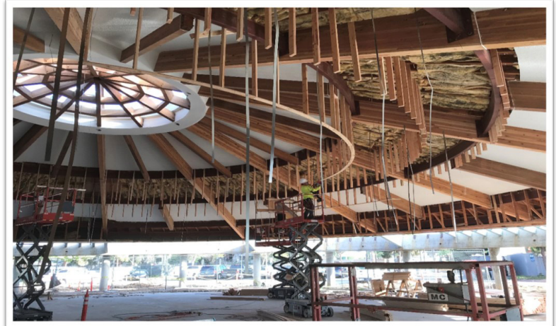
Renovations underway transforming an old library into the Norma Hertzog Community Center. This multi-purpose room features a skylight to reduce heat gain.
